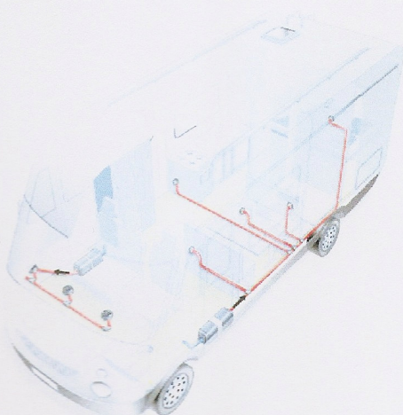
TYPICAL AIR HEATER SYSTEM LAYOUT
