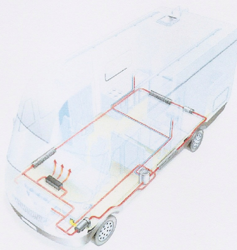
TYPICAL WATER HEATER SYSTEM LAYOUT
